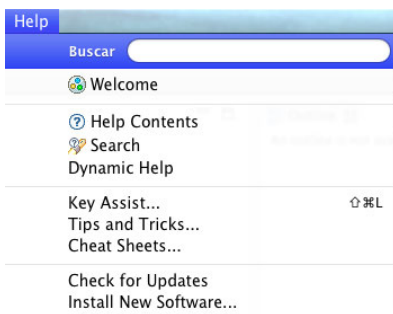
Figura 1.5: Menu Help
